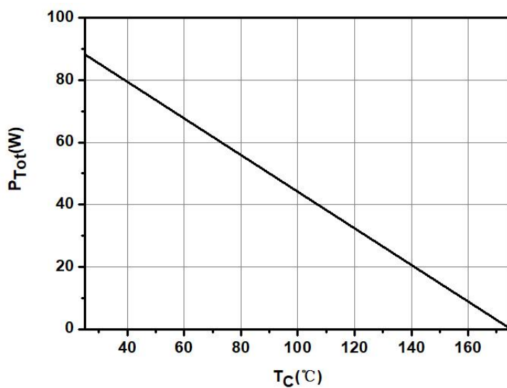
Fig.7-Power Derating
