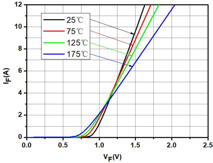
Fig.1-Typical Forward Voltage
